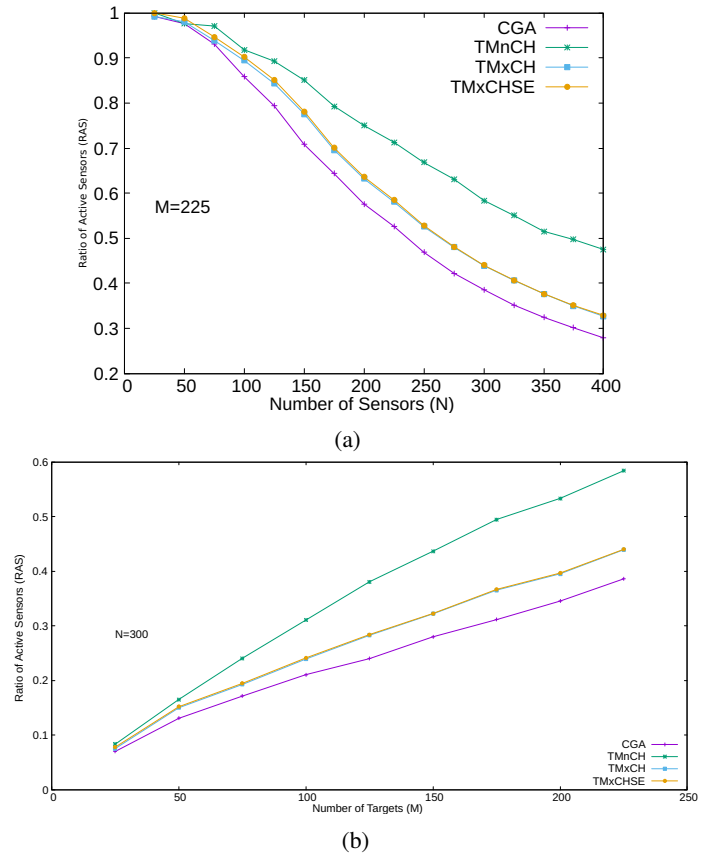
Figure 7: Sensor usage comparison of CGA, TMnCH, TMxCH and TMxCHSE heuristics
