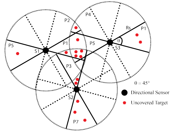
Figure 3: An example scenario
